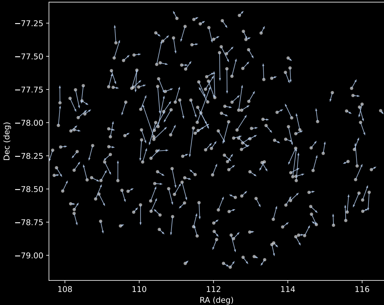
GALAH DR4 Cluster 1 Proper Motion Vectors (n=224)
