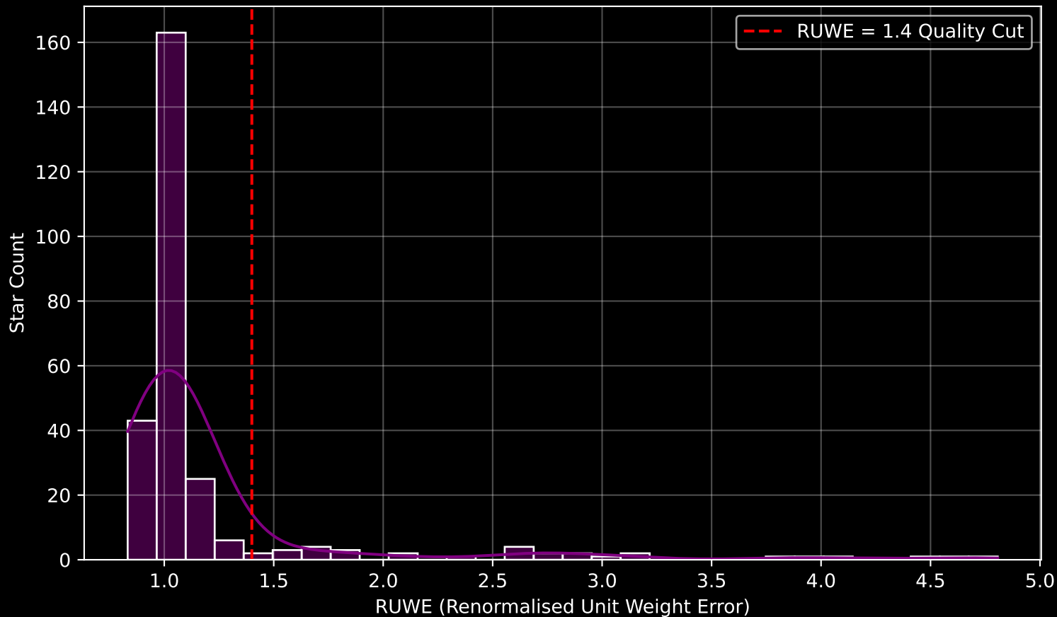
GALAH DR4 Field [250] RUWE Distribution (n= 269)
