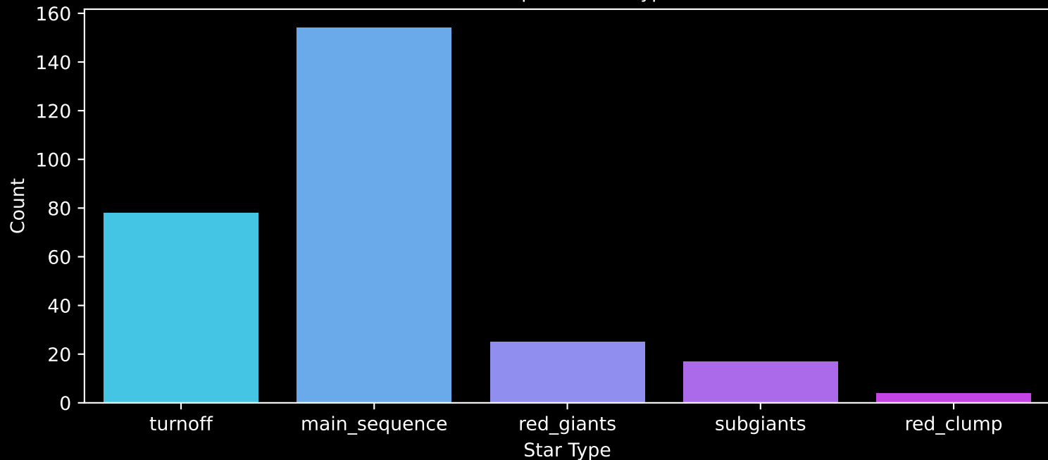
GALAH DR4 Field: [250] Count plot of Star Type
